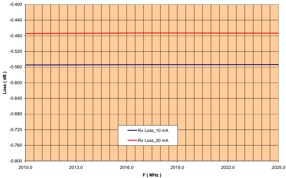
MASW-000823-12770T Ant-Rx Insertion Loss vs Frequency and Current
